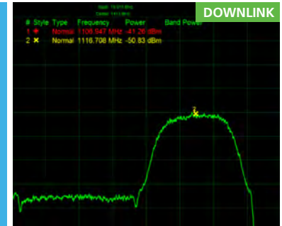
Fig. 6: Nominal Uplink & Downlink Spectrums for In-Beam Interferer Testing
