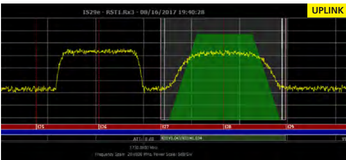
Fig. 11: Intelsat Epic Satellite Reconfigured to Terminate Interferer & Reallocate Friendly Carrier
