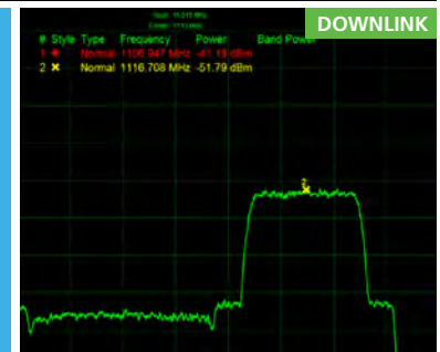
Fig. 7: In-Beam Interferer Only Spectrums
