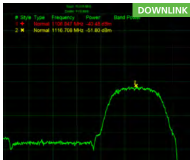
Fig. 11: Intelsat Epic Satellite Reconfigured to Terminate Interferer & Reallocate Friendly Carrier
